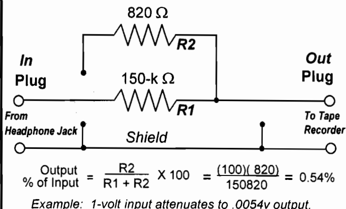
FIGURE 7: AUDIO DUBBING ADAPTER
