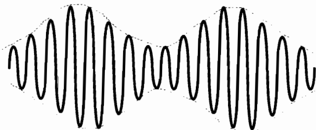
B. Amplitude modulated (AM) RF carrier wave
