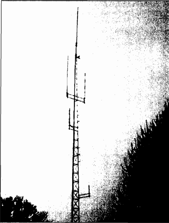
Typical public safety base antenna system Note that all antennas are vertically polarized
