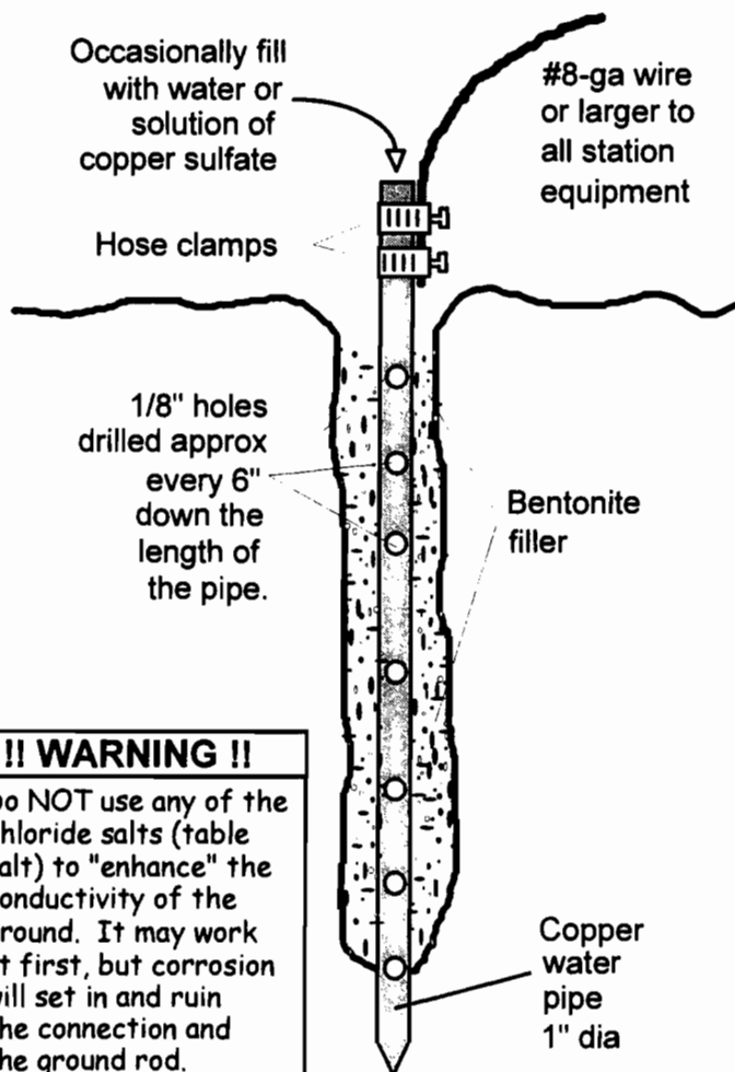
FIGURE 18: AN EFFECTIVE GROUND
