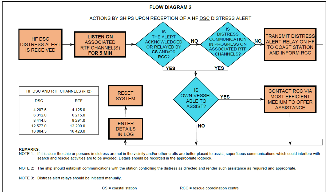
Figure 4-11 - Flow Diagram 2
